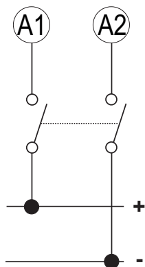
Fig. 1 Power supply
